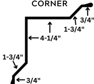
COMMERCIAL INSIDE CORNER
