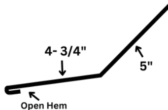
FF100 LOWER GAMBREL
