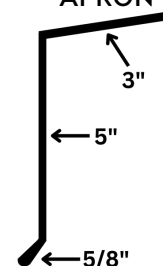
COMMERCIAL GUTTER APRON
