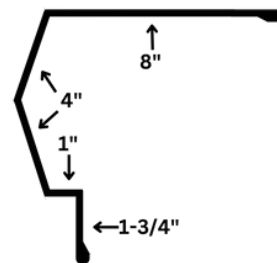
COMMERCIAL JAMES POST HUNG
