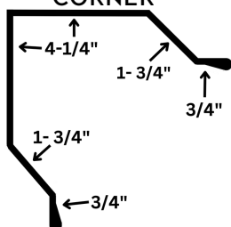
COMMERCIAL OUTSIDE CORNER
