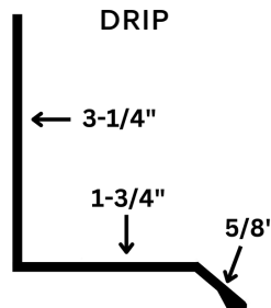
COMMERCIAL WINDOW DRIP
