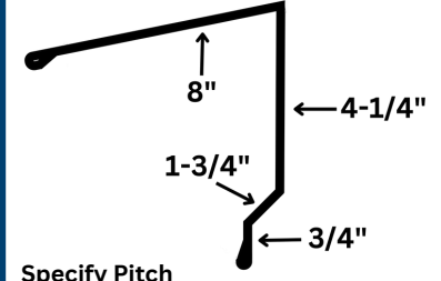
COMMERCIAL HIGH SIDE
