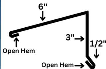
FF100 VENTED J CLEAT
