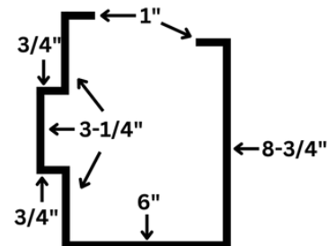
COMMERCIAL LOWER GAMBREL
