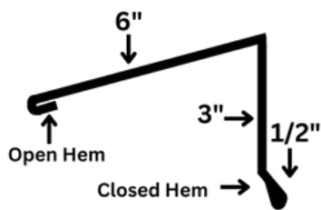
FF100 Z CLEAT
